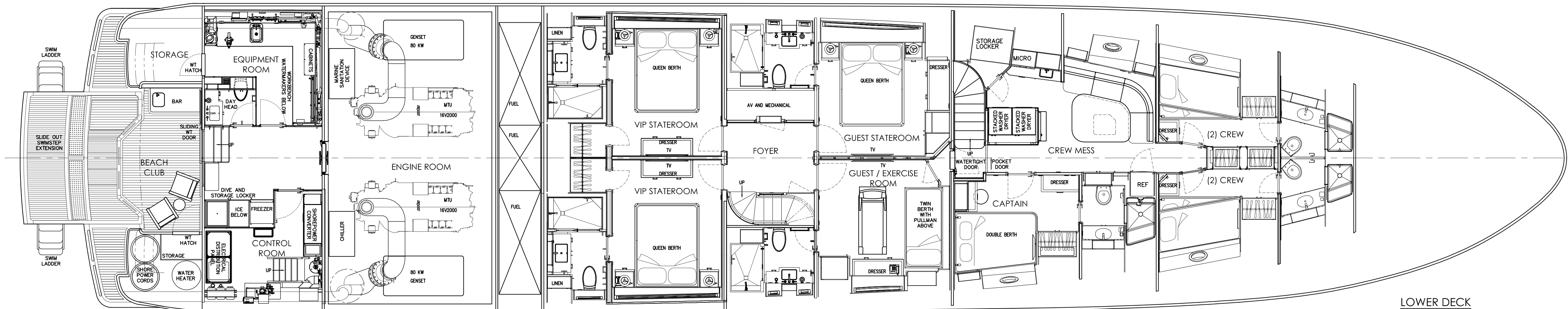
LOWER DECK
